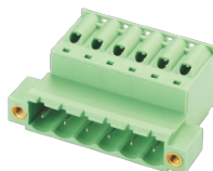
WJ2EDGVHM-5.0/5.08
