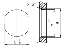
Panel cut-out
