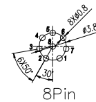
8Pin
